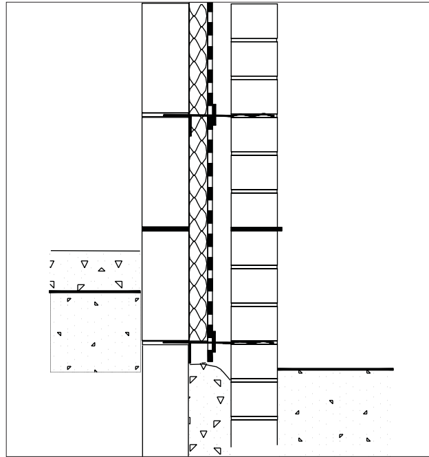
Figure 2 Installation of wall ties
