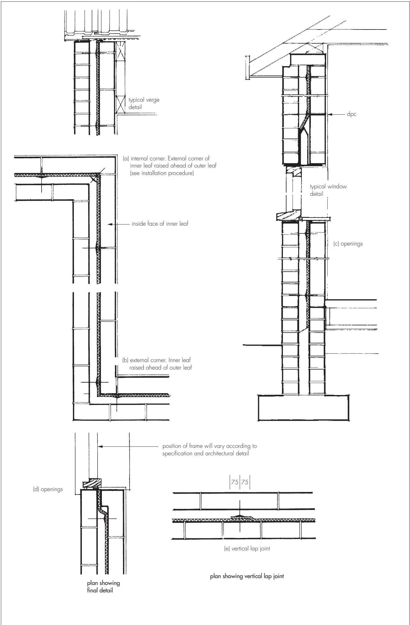
Figure 4 Fixing details (dimensions in mm)
